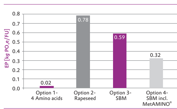
Figure 6-2 Eutrophication potential EP [CML 2001] of broiler production.
