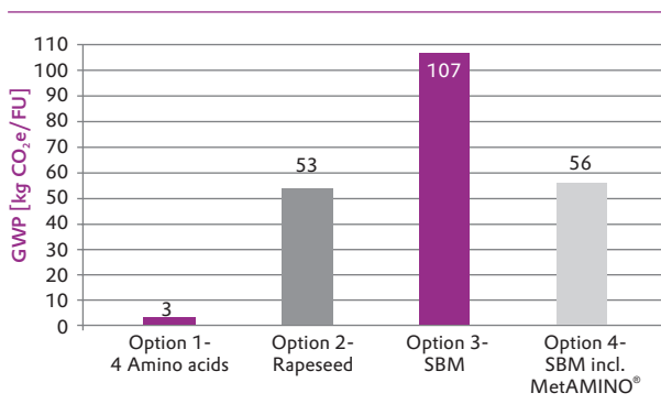
Figure 5-2 Global warming potential GWP100 [CML 2001] of broiler production.
