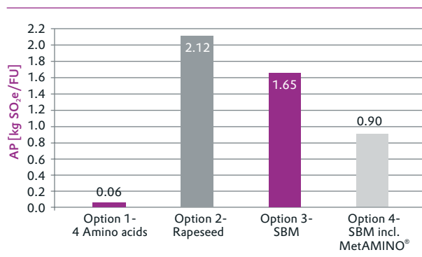
Figure 7-2 Acidification potential AP [CML 2001] of broiler production.
