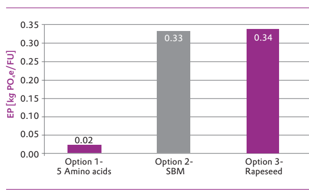
Figure 6-1 Eutrophication potential EP [CML 2001] of pig production.
