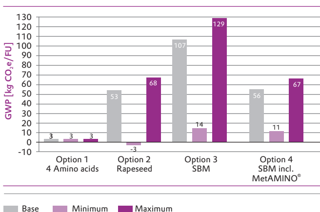
Figure 8 GWP [CML 2001] from broiler production – sensitivity analysis for “land use change soya”
