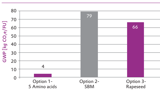
Figure 5-1 Global warming potential GWP100 [CML 2001] of pig production.
