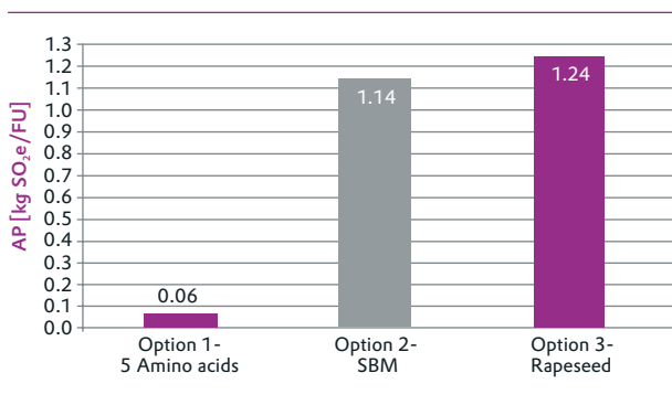
Figure 7-1 Acidification potential AP [CML 2001] of pig production.
